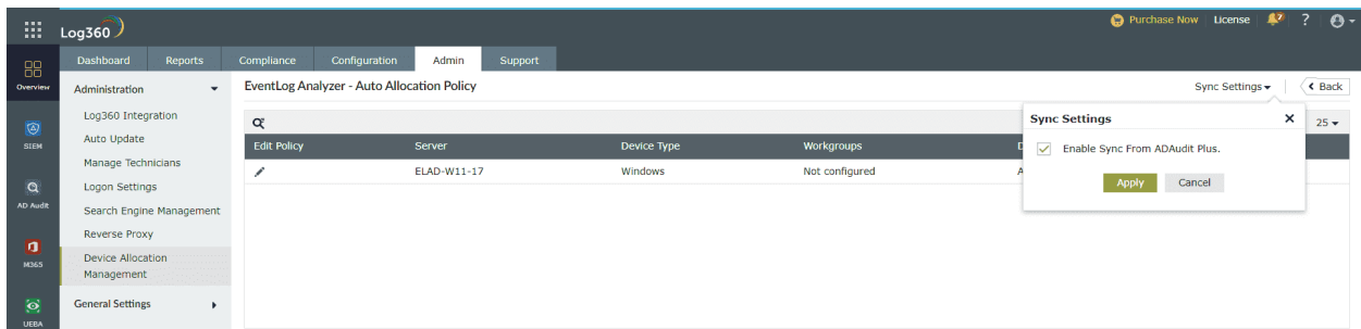
Figure 56 Sync settings
