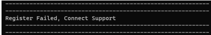
Fig 17 Conversion failed
