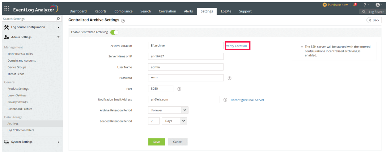
Figure 33 Verify Location
