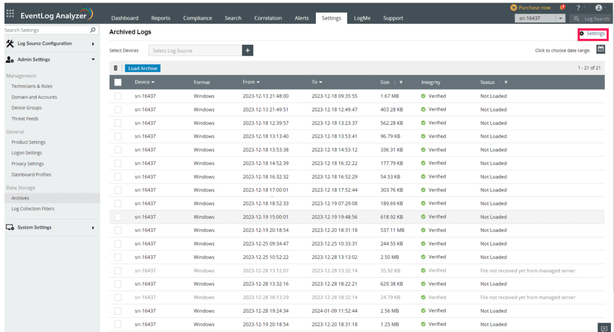
Figure 30 Settings
