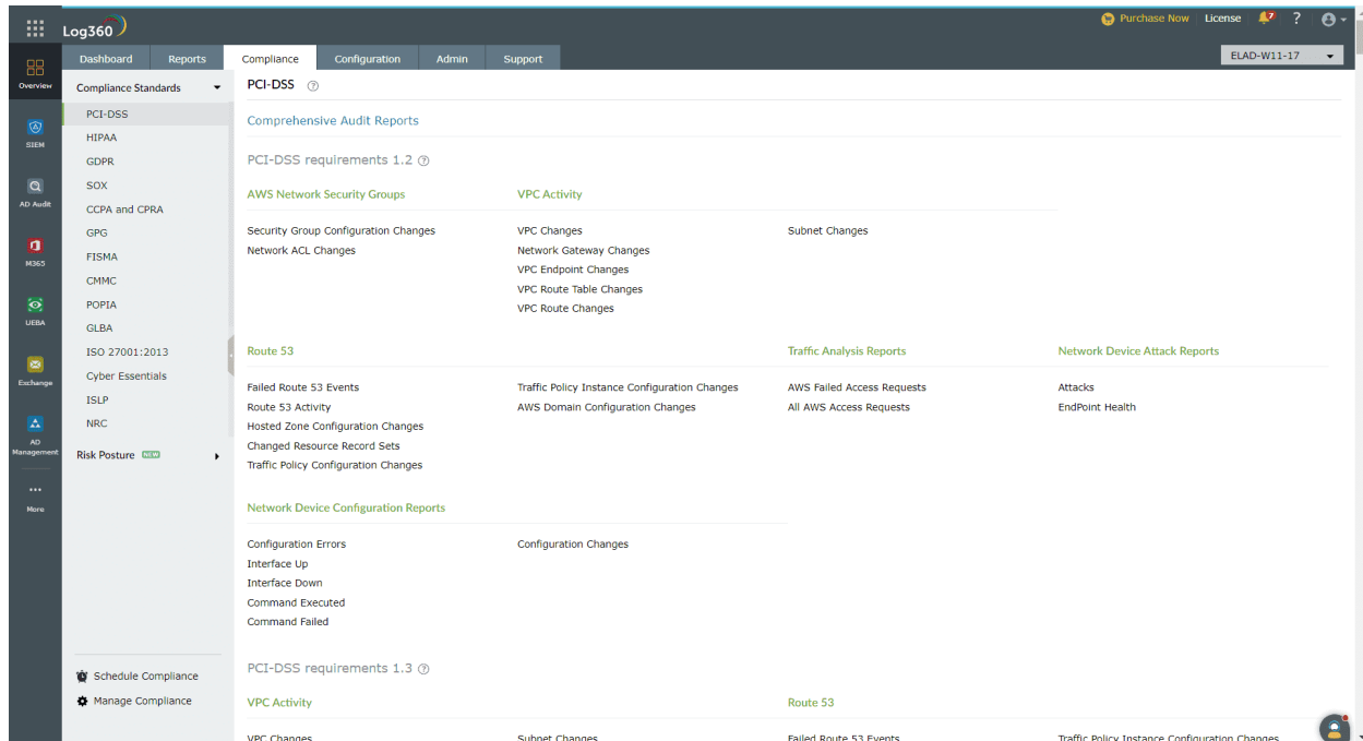
Figure 57 Compliance Standards
