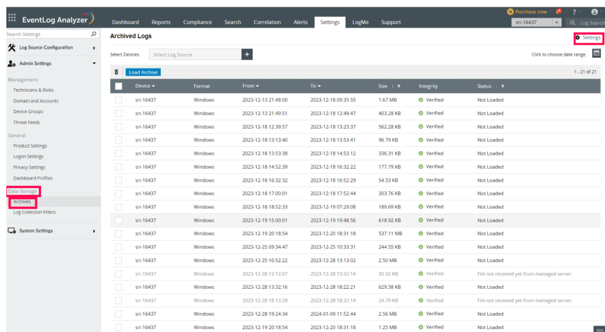
Figure 29 Archived Logs
