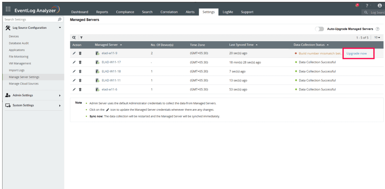
Fig 27 Upgrade now
