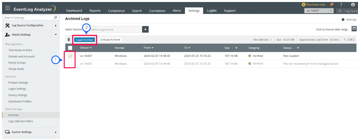
Figure 43 Load Archive
