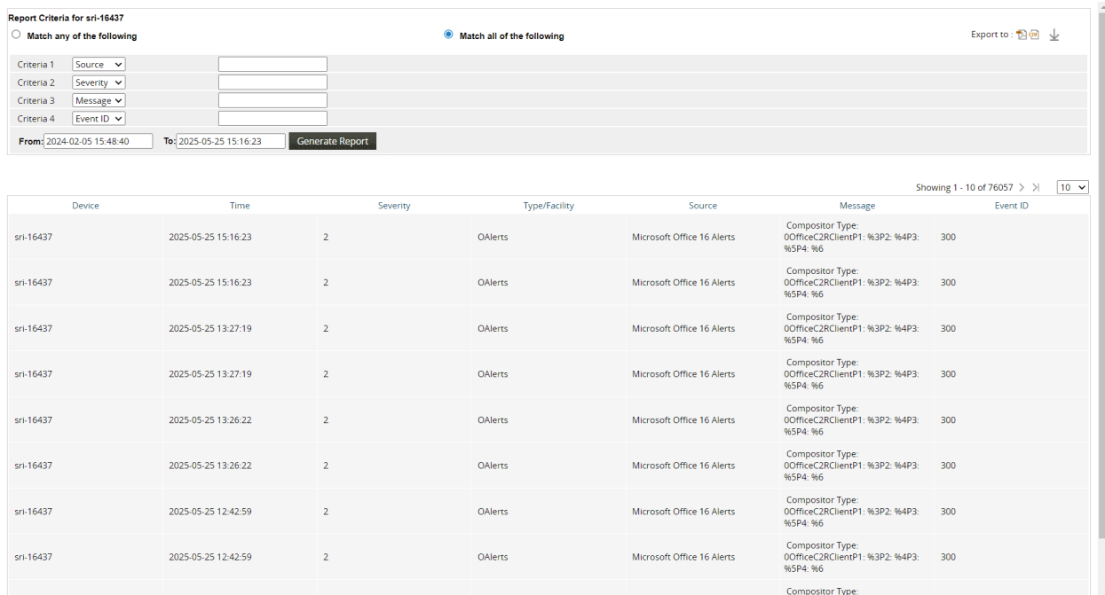
Figure 45 Reports
