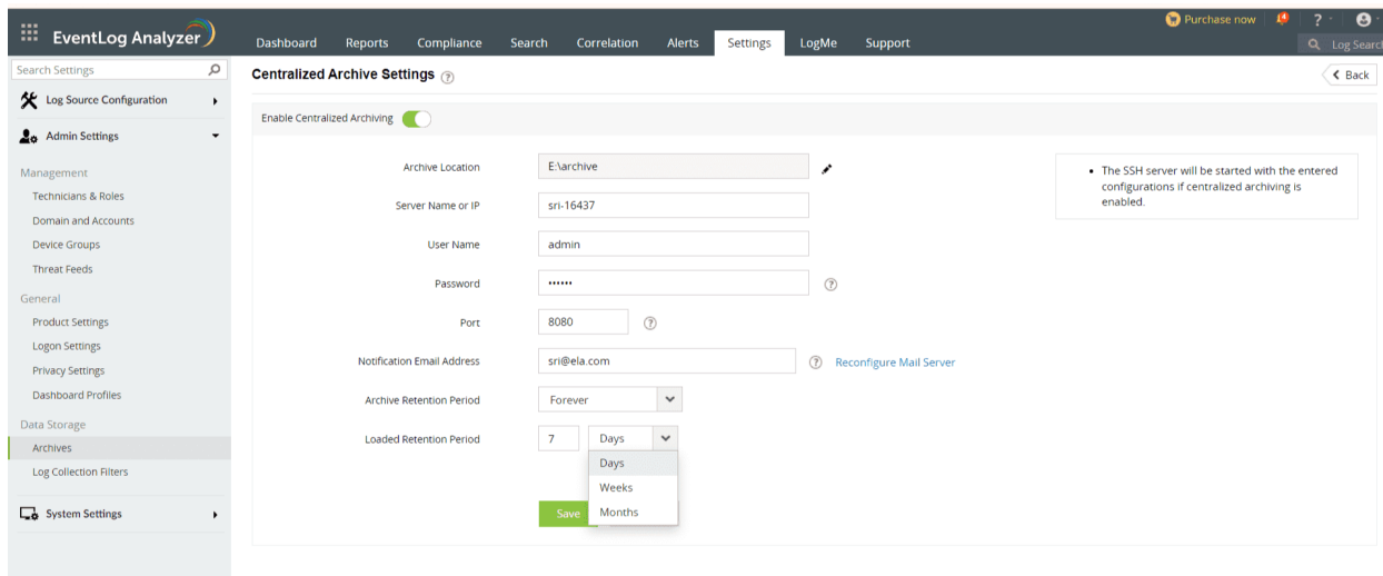
Figure 42 Save
